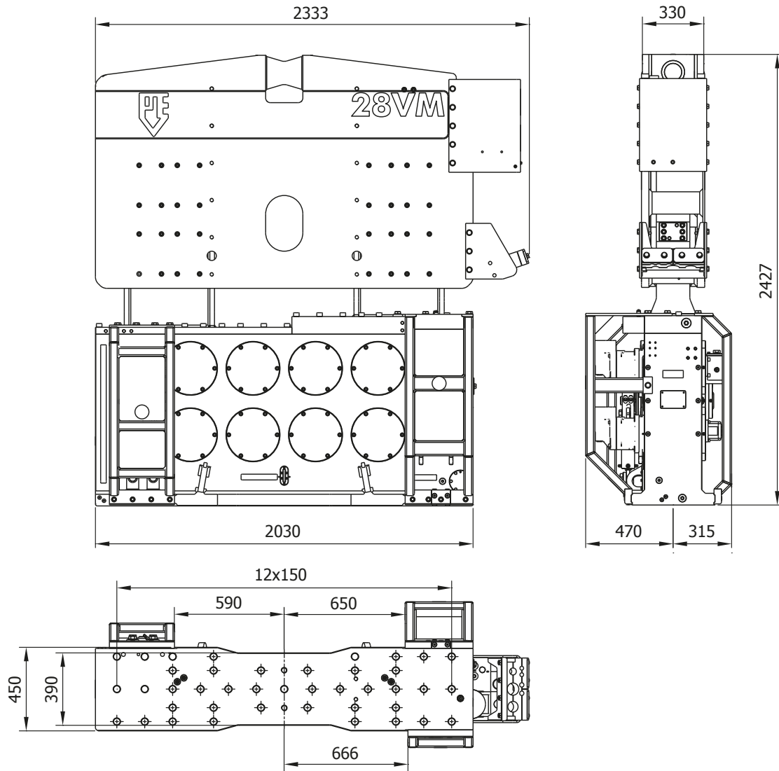
dimension in mm
